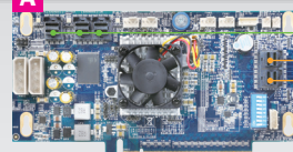
12Gb/s SAS expander controller
